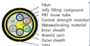
ADSS Aerial Cable
